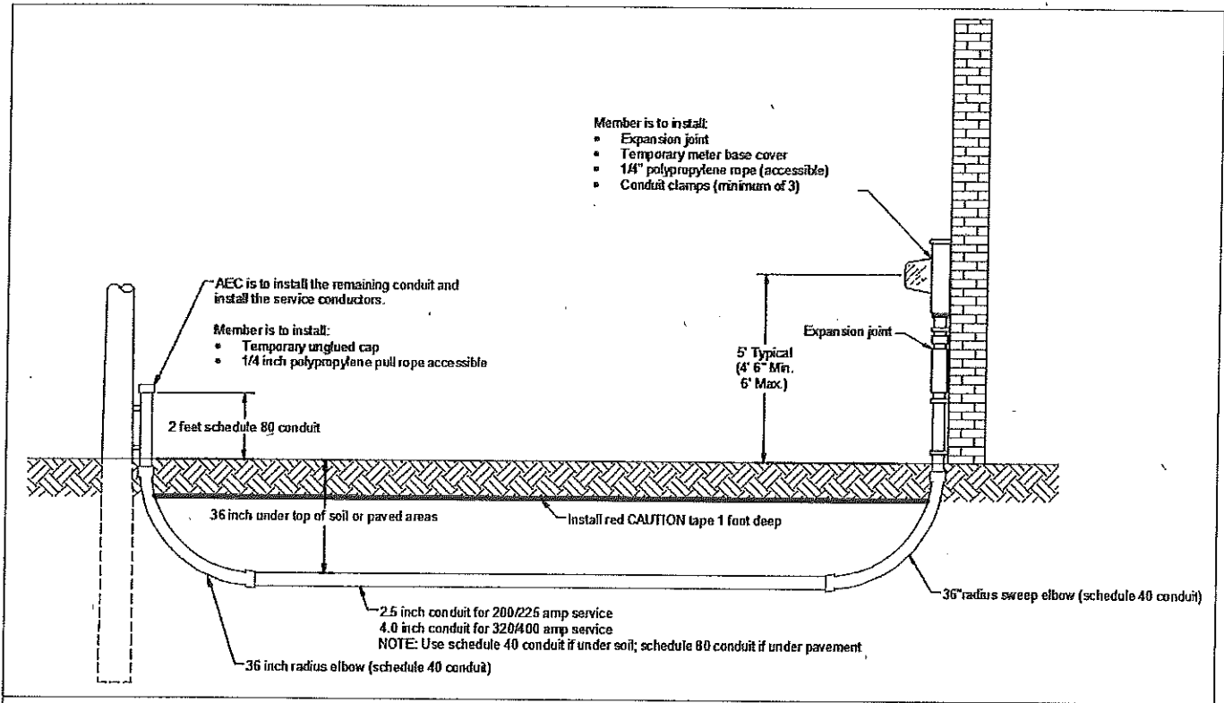
Pole Mounted Transformer to Meter Base Installation
