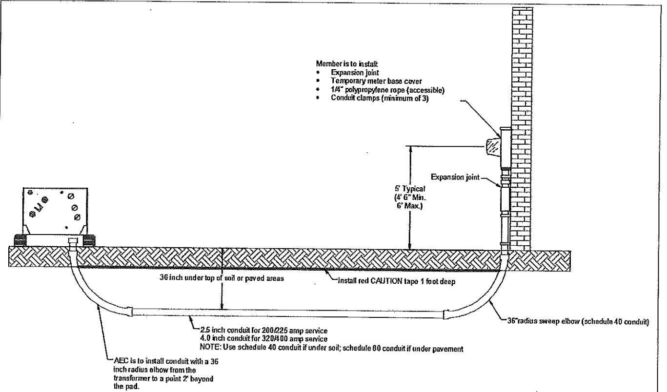
Padmounted Transformer to Meter Base Installation
